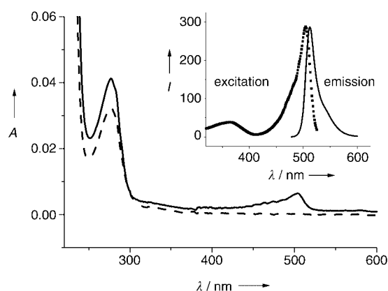
Figure 2. Absorption spectra of DsbC labeled with BODIPY. DsbC ( 1 ) was modified in the presence (solid line, 4 , 1.2 μM) and absence (dashed line, 1.0 μM) of glyoxylate. The inset shows the excitation ( \lambda_{\text{em}} = 535 nm) and emission ( \lambda_{\text{ex}} = 467 nm) spectra of 4 (4.1 μM); 5-nm excitation and emission slits were used.
