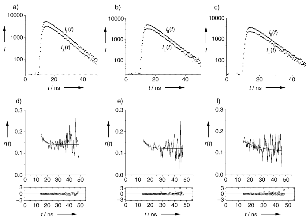
Figure 3. a)–c) Polarized fluorescence decays of I_{\parallel}(t) and I_{\perp}(t) and d)–f) anisotropy decays (along with the best-fit curves and the weighted residuals) of 4 (4.1 \mu M) at various extents of denaturing of the DsbC protein; a), d) native DsbC; b), e) denatured in GuHCl (1.5 M); c), f) denatured in GuHCl (6 M) with dithiothreitol (DTT, 0.1 M). I_{\parallel}(t) and I_{\perp}(t) represent the intensities of the fluorescence observed with the emission polarizer oriented parallel and perpendicular, respectively, to the excitation polarizer. All measurements were carried out at 273 K.
