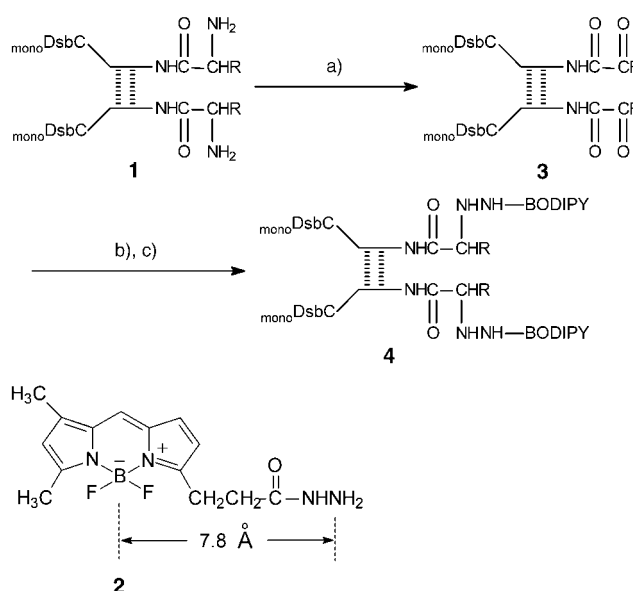
Figure 1. Specific modification of the N-terminal amino groups of dimeric DsbC ( 1 ): a) transamination reaction with glyoxylate; b) coupling with 2 ; c) reduction with sodium cyanoborohydride. The separation between the central B atom of the BODIPY FL dye and the terminal N atom of the hydrazide group of the linker arm in 2 is 7.8 Å (calculated with CS Chem 3D software). BODIPY FL = 4,4-difluoro-5,7-dimethyl-4-bora-3a,4a-diaza-s-indacene-3-propionic acid.
